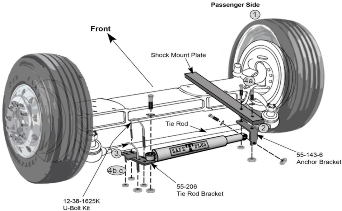
Safe T Plus Instal lation Diagr am
